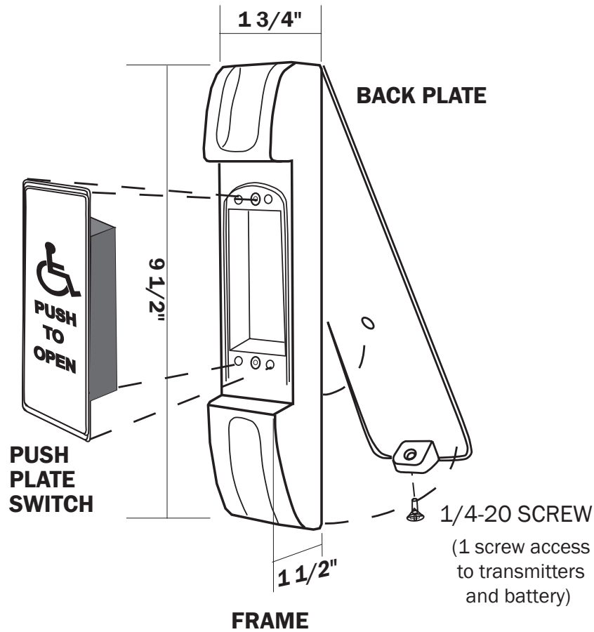
CP/TX-J Radio Transmitter (Pictured with 59J-H—Sold Separately)
