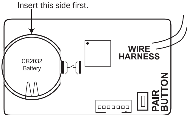
FIGURE 2 Transceiver Circuit Board
